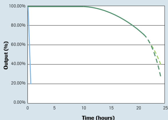
Chart 1: Affects of 10ppm HMDS on sensor output
