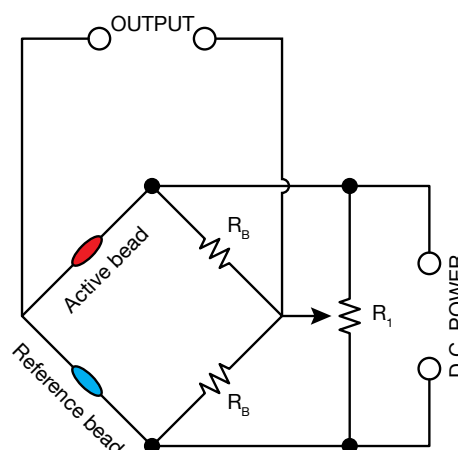
Fig 1: Wheatstone bridge circuit diagram
