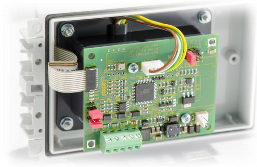
Figure 4: 4-pin data cable connecting the IR sensor to the interface PCB
