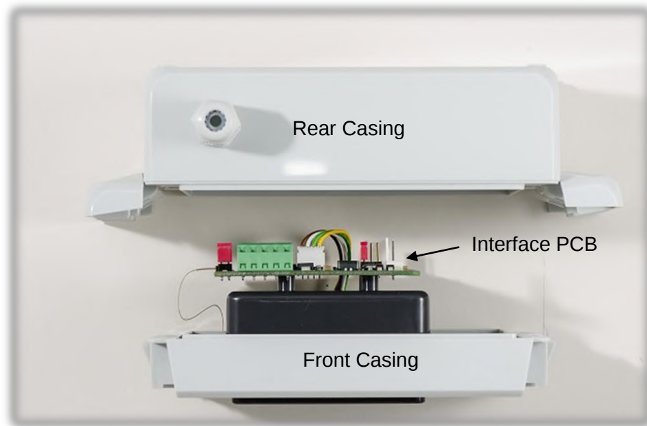
Figure 1: F-Gas Detector Layout
