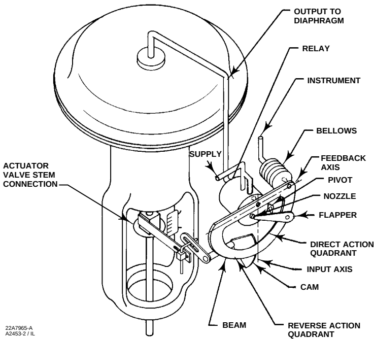
Figure 4-2. Positioner Schematic for Diaphragm Actuator
