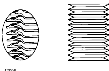
Figure 3-20. Welded Leaf Bellows
