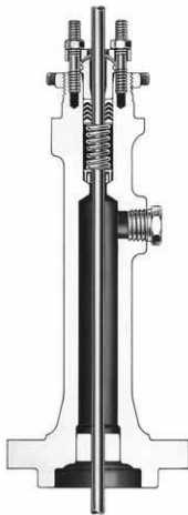
Figure 1-5. Extension Bonnet
