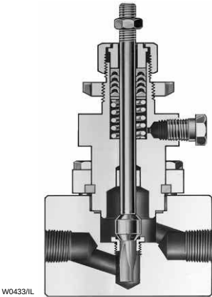
Figure 3-3. Bar Stock Valve Bodies
