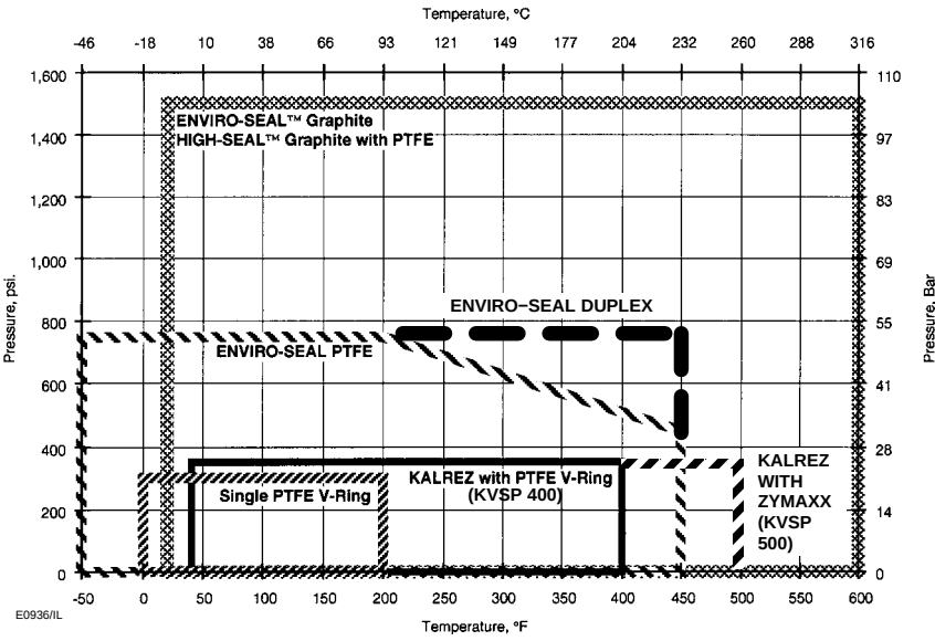
Figure 5-15. Application Guidelines Chart for 100 PPM Service
