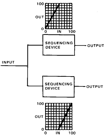
SIGNAL AMPLITUDE SEQUENCING (SPLIT-RANGING)
