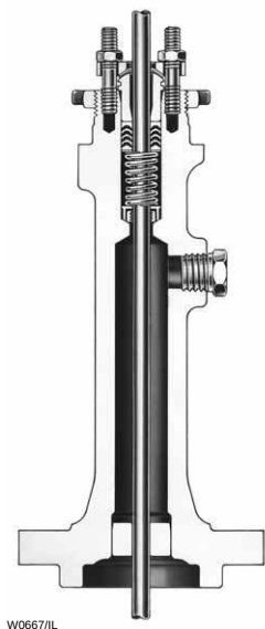
Figure 6-3. Typical Extension Bonnet
