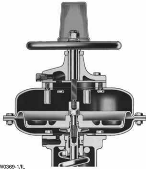
Figure 4-6. Top-Mounted Hand-wheel for Reverse-Acting Diaphragm Actuator
