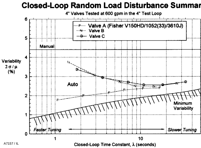
Figure 2-7. Closed-Loop Performance
