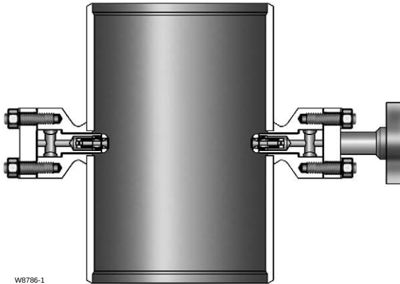
Figure 7-11. Steam Cooler
