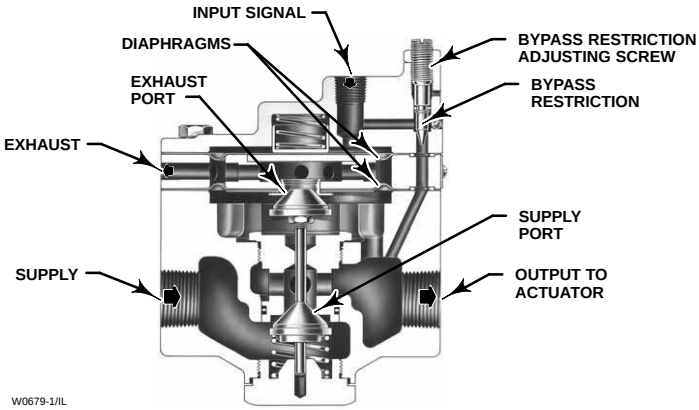
Figure 4-4. Volume Booster
