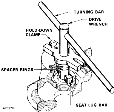
Figure 8-6. Seat Ring Puller
