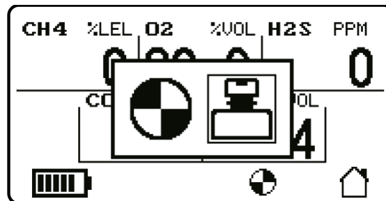
Figure 15: Bump/Pump screen
