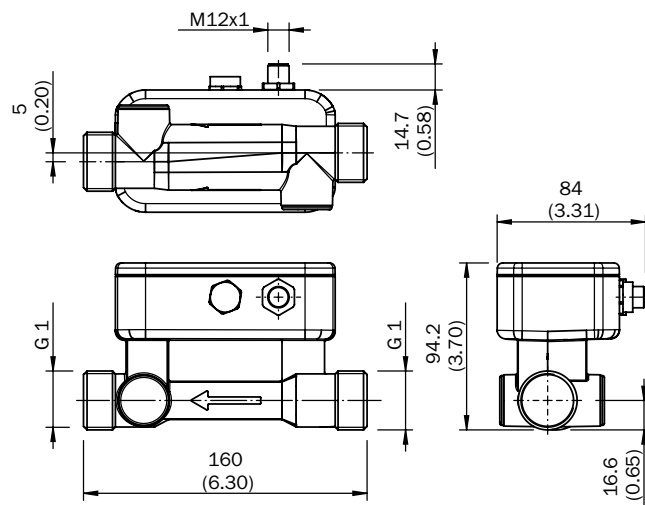
NW 20, G 1
