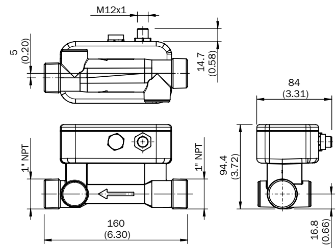
NW 20, 1" NPT
