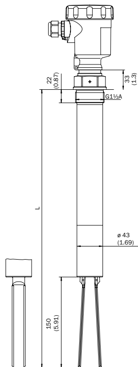
LBV330 threaded version G 1 ½ A (DIN ISO 228/1)
