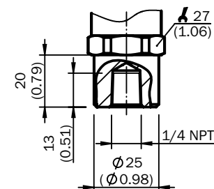
1/4" NPT female
