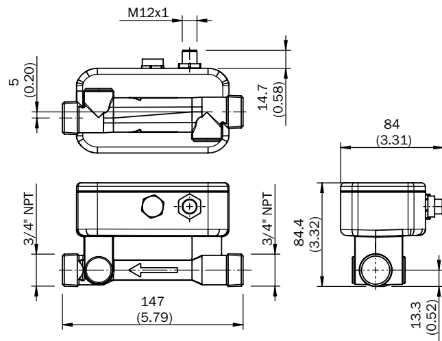
NW 15, 3/4" NPT
