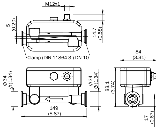
NW 10, Clamp (DIN 11864-3)
