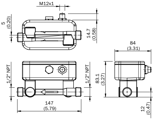
NW 10, 1/2" NPT
