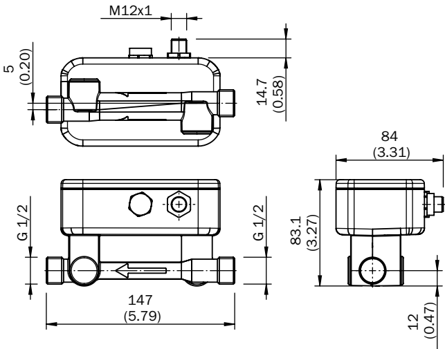
NW 10, G 1/2
