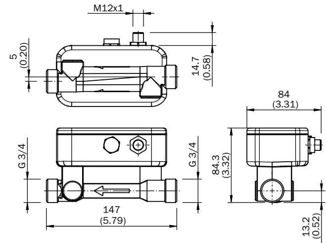
NW 15, G 3/4
