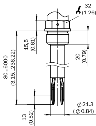
G 1 A, 1" NPT
