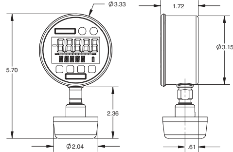
Types 2136, 2236 with 1½" inline seal
