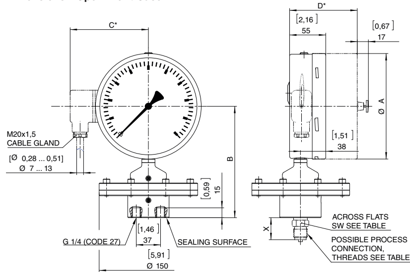
Dimensions - Open Front Case
