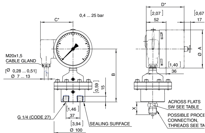
Dimensions - Solid Front Case
