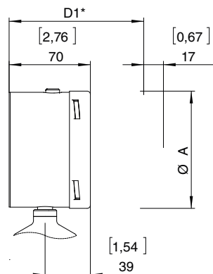
Dimensions - Solid Front Case
