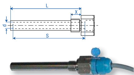
Thermowell fitted with sealing holes
