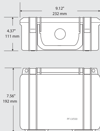
ELECTRONICS ENCLOSURE
