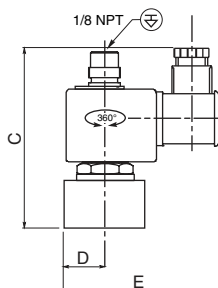
TYPE 09: WP / WS EM / WSEM Steel; epoxy coated / AISI 316 SS IEC 335/EN 60079-7/18 and EN 61241-1
