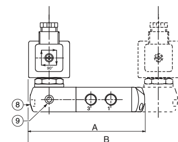
TYPE 09: WP / WS EM / WSEM Steel; epoxy coated / AISI 316 SS IEC 335/EN 60079-7/18 and EN 61241-1
