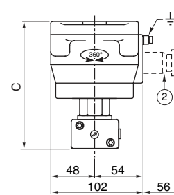
TYPE 10: PV Epoxy encapsulated EN/IEC 60079-18 and EN/IEC 61241-18
