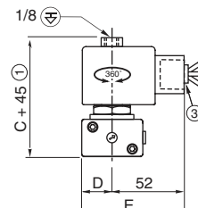
TYPE 08: NF / WSNF Aluminium; epoxy coated / AISI 316L SS EN/IEC 60079-1 and EN/IEC 60079-31
