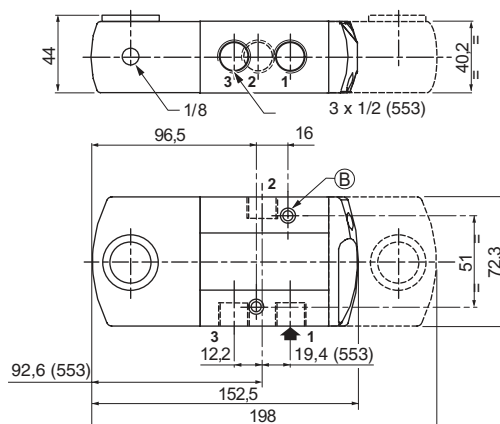
TYPE 02: NF / WSNF Aluminium; epoxy coated / AISI 316L SS EN/IEC 60079-1 and EN/IEC 60079-31
