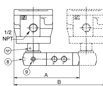
TYPE 10: PV Epoxy encapsulated EN/IEC 60079-18 and EN/IEC 61241-18
