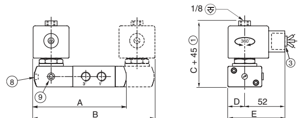
TYPE 08: NF / WSNF Aluminium; epoxy coated / AISI 316L SS EN/IEC 60079-1 and EN/IEC 60079-31
