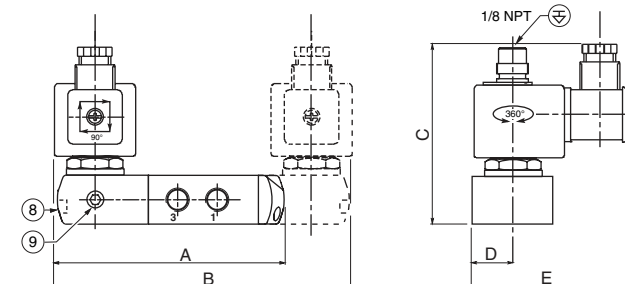
TYPE 09: WP / WS EM / WSEM Steel; epoxy coated / AISI 316 SS IEC 335/EN 60079-7/18 and EN 61241-1
