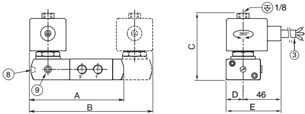
TYPE 07: SC Epoxy moulded IEC 335 / ISO 4400
