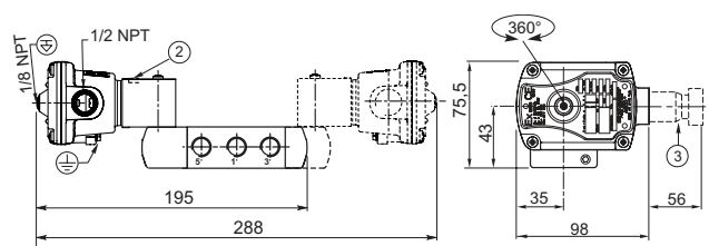
TYPE 03: No prefix, IP65 [suffixes 551: GD (II 1 GD c) ; SL (SIL) ; GDSL (SIL, II 1 GD c) suffix 553: GD (II 2 GD c) ; SL (SIL) ; GDSL (SIL, II 2 GD c)] Air operated version
