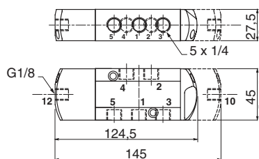
TYPE 03: No prefix, IP65 [suffixes 551: GD (II 1 GD c) ; SL (SIL) ; GDSL (SIL, II 1 GD c) suffix 553: GD (II 2 GD c) ; SL (SIL) ; GDSL (SIL, II 2 GD c)] Air operated version
