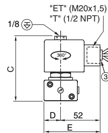
TYPE 06: EF and EV: NEMA type 7 and 9 Epoxy encapsulated ICS-6 ANSI NOTE: applicable to solenoid only
