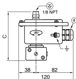
TYPE 09: WP / WS EM / WSEM Steel; epoxy coated / AISI 316 SS IEC 335 / EN 60079-7/18 and EN 61241-1
