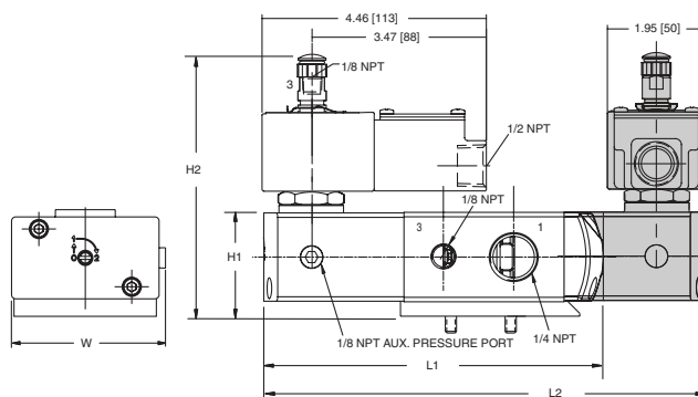
8551 NAMUR Footprint
