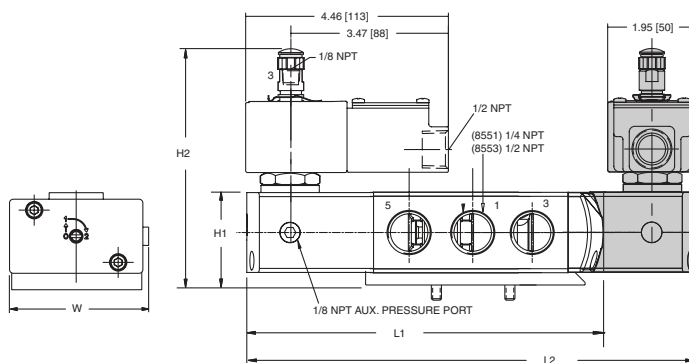
8553 NAMUR Footprint
