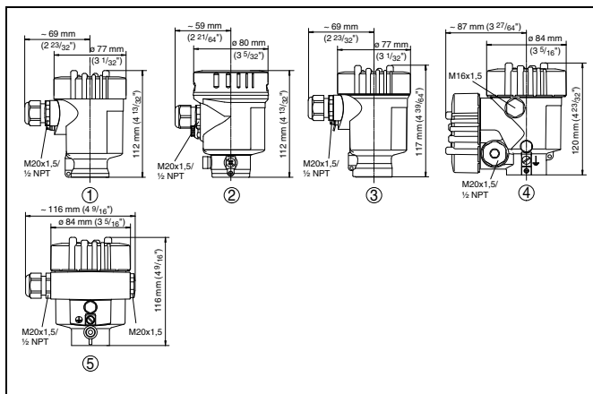
Fig. 23: Housing versions
