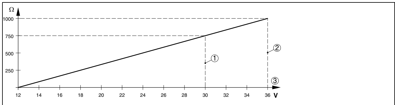
Fig. 22: Voltage diagram > 4 ... < 20 mA - for connection to a signal conditioning instrument
