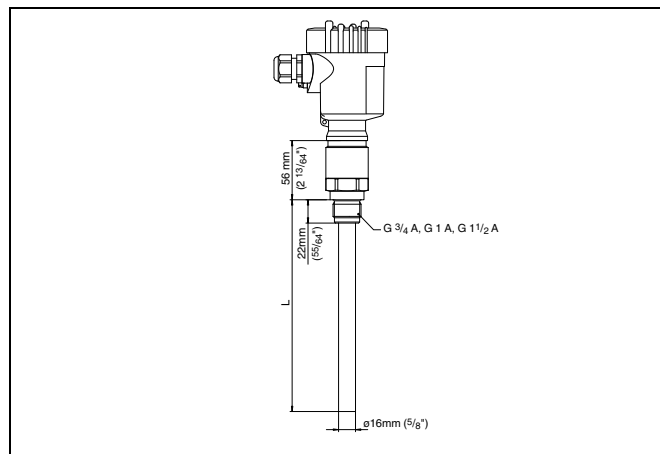
Fig. 26: VEGACAL 63 - threaded version
