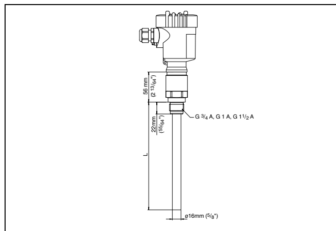
Fig. 28: VEGACAL 64 - threaded version
