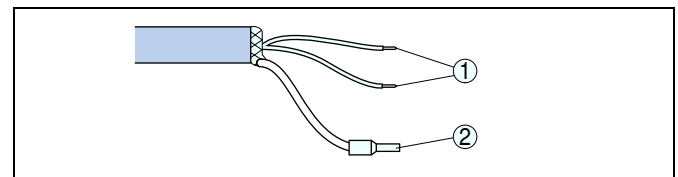
Fig. 20: Wire assignment fix-connected connection cable
