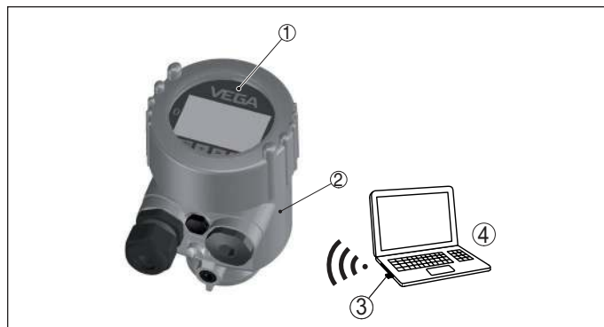
Fig. 32: Connection of the PC via Bluetooth adapter
