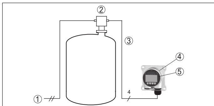
Fig. 33: Connection of VEGADIS 81 to the sensor
