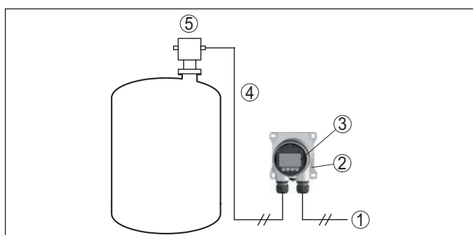
Fig. 34: Connection of VEGADIS 82 to the sensor
