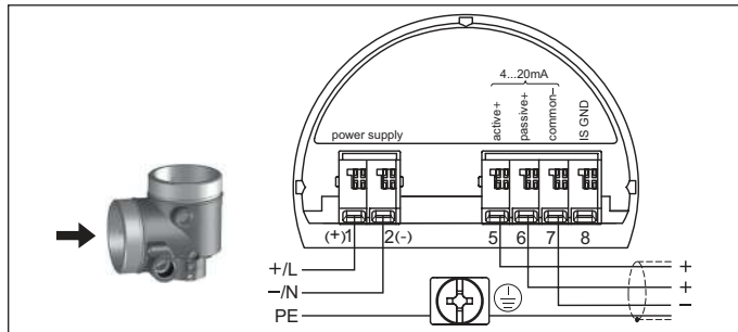
Fig. 22: Terminal compartment, double chamber housing
