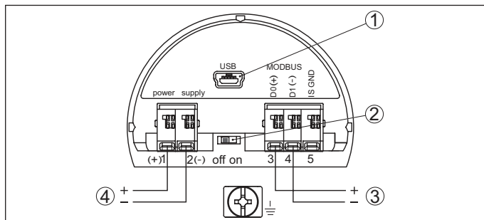
Fig. 27: Terminal compartment
