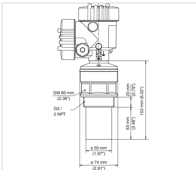
Dimensions VEGASON 62
