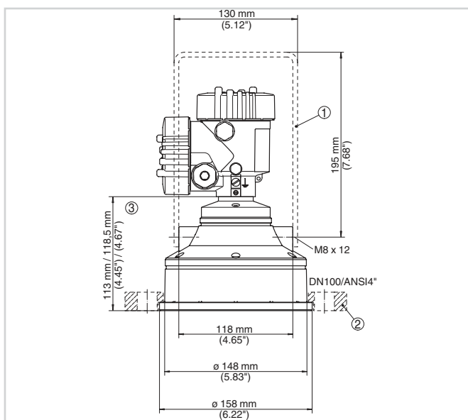
Dimensions VEGASON 63
