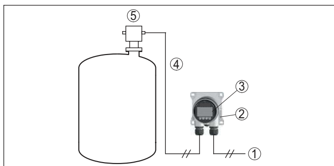
Fig. 38: Connection of VEGADIS 82 to the sensor
