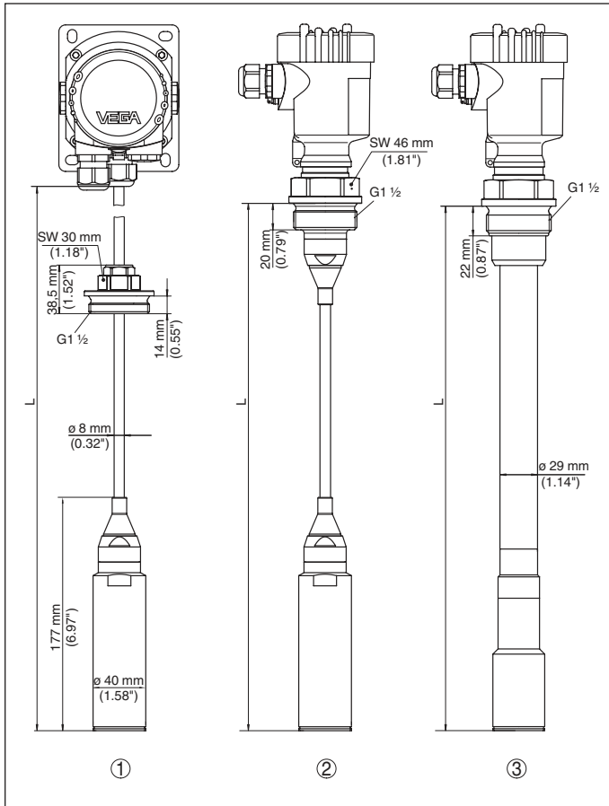
Fig. 46: Dimensions VEGABAR
