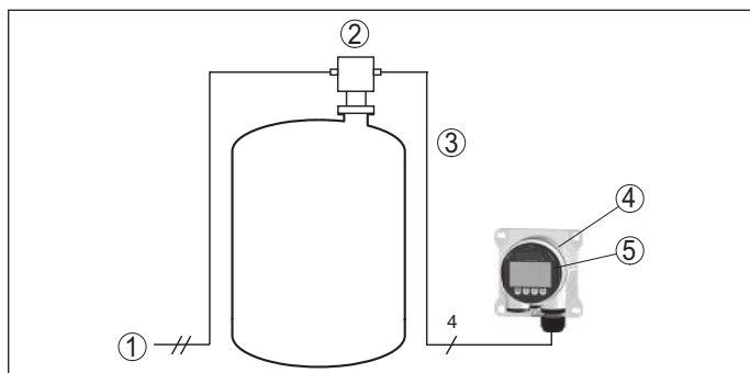
Fig. 37: Connection of VEGADIS 81 to the sensor
