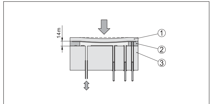
Fig. 3: Configuration of the CERTEC® measuring cell in VEGAWELL 52
