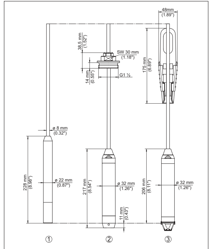
Fig. 46: Dimensions VEGABAR
