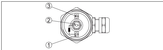
Fig. 6: Terminal compartment
