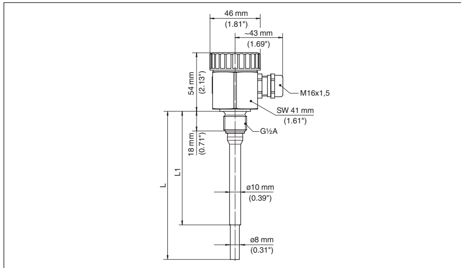
Fig. 9: Conductive rod electrode EL 1
