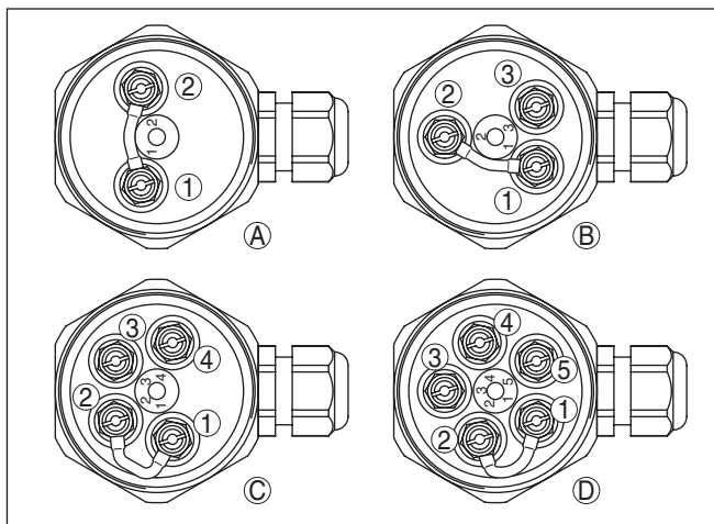
Fig. 4: Connection compartment of the probe - 220 k \Omega resistance between terminals 1 and 2
