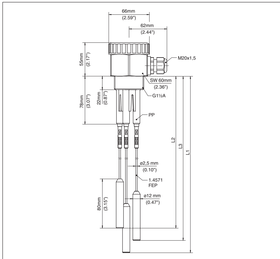
Fig. 7: Conductive multiple cable electrode EL 6
