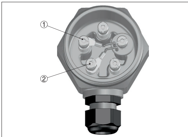
Fig. 6: Mounting of the additional electronics for line break monitoring
