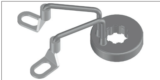
Fig. 5: Supplementary electronics for line break monitoring in conjunction with VEGATOR 632
