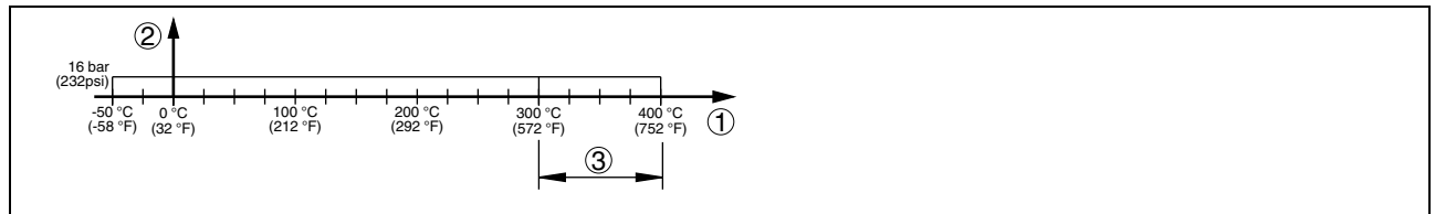
Fig. 17: VEGACAP 67 - process temperature - process pressure
