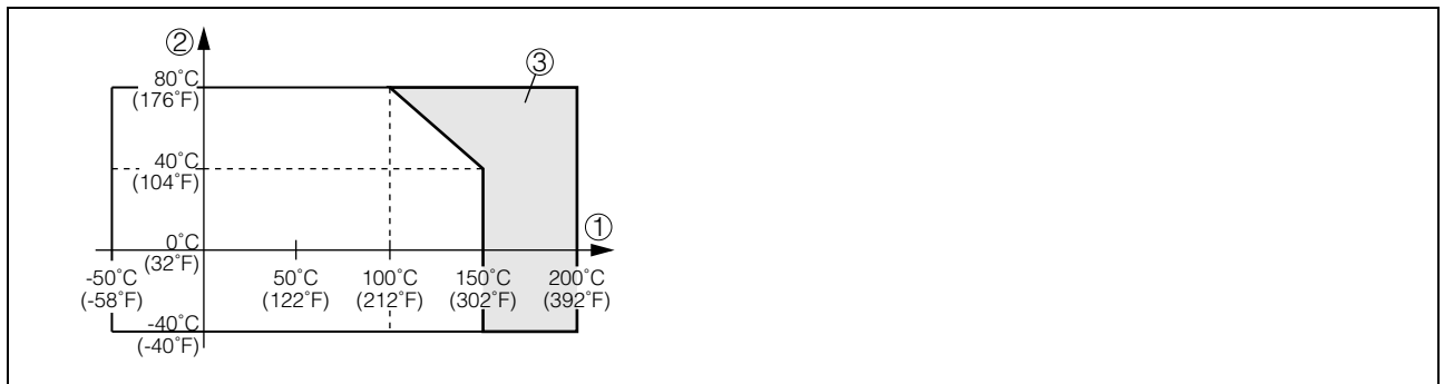
Fig. 16: VEGACAP 62, 65, 65 - ambient temperature - product temperature
