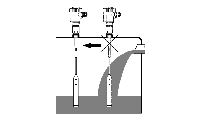
Fig. 5: Inflowing medium
