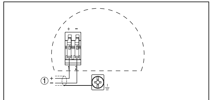
Fig. 11: Wiring plan, single chamber housing
