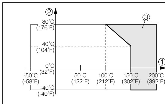
Fig. 13: VEGACAP 62, 63, 64, 66 - ambient temperature - product temperature
