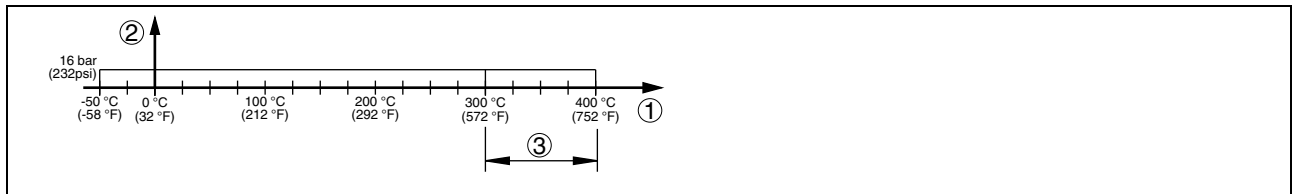
Fig. 17: VEGACAP 67 - process temperature - process pressure
