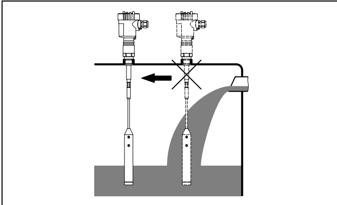
Fig. 8: Inflowing medium
