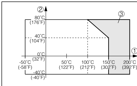
Fig. 16: VEGACAP 62, 65, 65 - ambient temperature - product temperature
