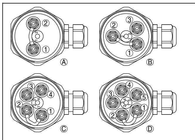
Fig. 13: Connection compartment of the probe - 220 kΩ resistor between terminals 1 and 2
