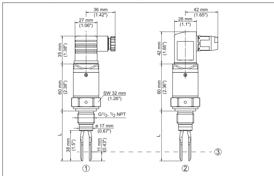
Fig. 32: VEGASWING 51, standard version - thread G\frac{1}{2} , \frac{1}{2} NPT
