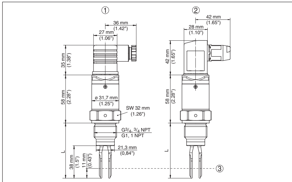
Fig. 33: VEGASWING 51, standard version - thread G \frac{3}{4} , G1 / \frac{3}{4} NPT, 1 NPT
