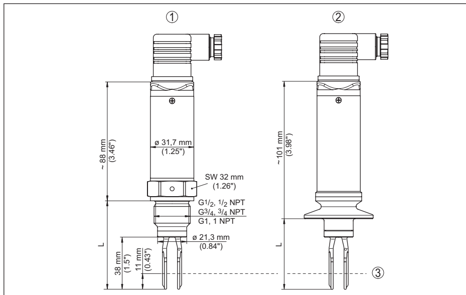
Fig. 34: VEGASWING 51, high temperature version
