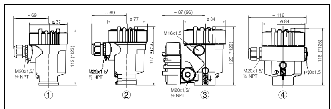
Fig. 50: Housing versions
