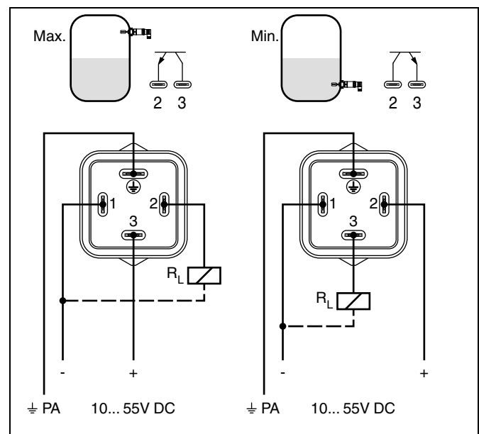
Fig. 19: VEGASWING 51 - transistor output with valve plug DIN 43650
