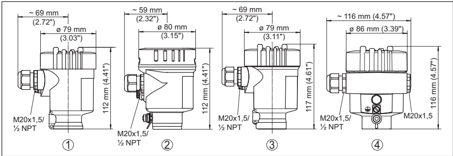
Fig. 29: Housing versions
