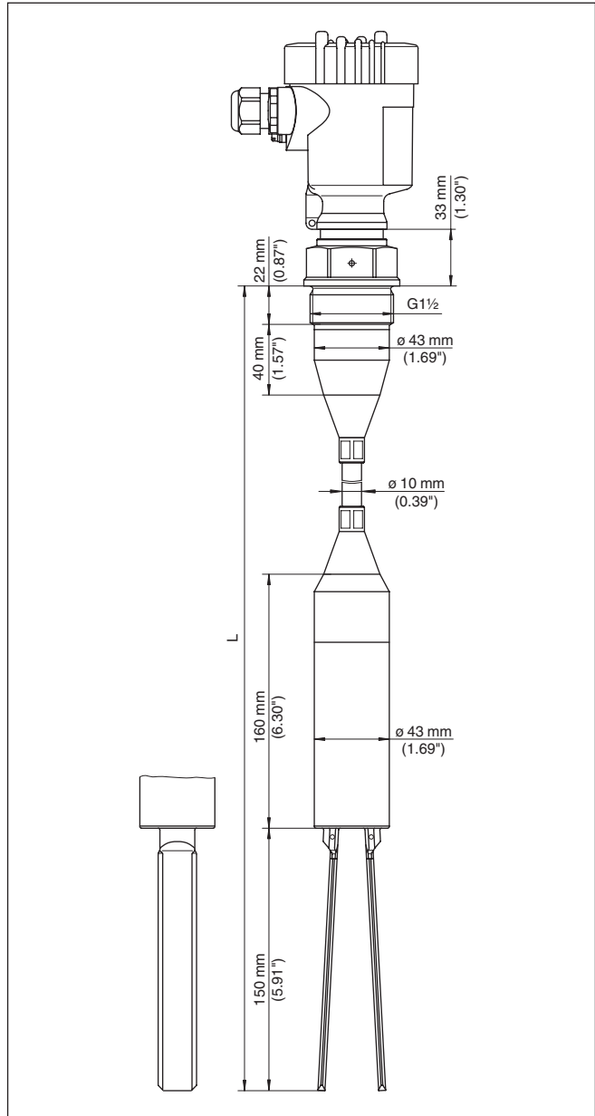
Fig. 31: VEGAWAVE 62 with FEP suspension cable, threaded version G1½ A (DIN ISO 228/1)
