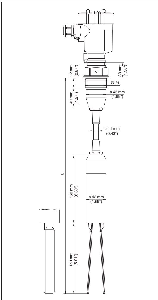
Fig. 30: VEGAWAVE 62 with PUR suspension cable, threaded version G1½ A (DIN ISO 228/1)
