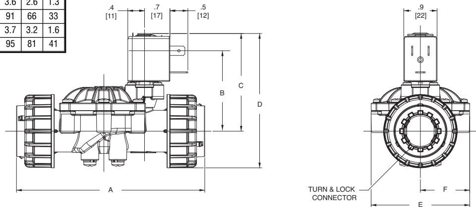
3/4" & 1" TURN & LOCK CONNECTION WITH DIN CONNECTION
