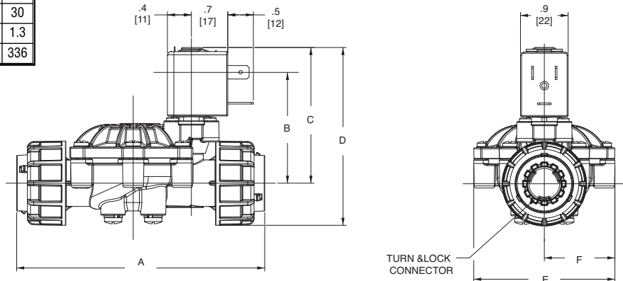
3/8" & 1/2" TURN & LOCK CONNECTION WITH DIN CONNECTION
