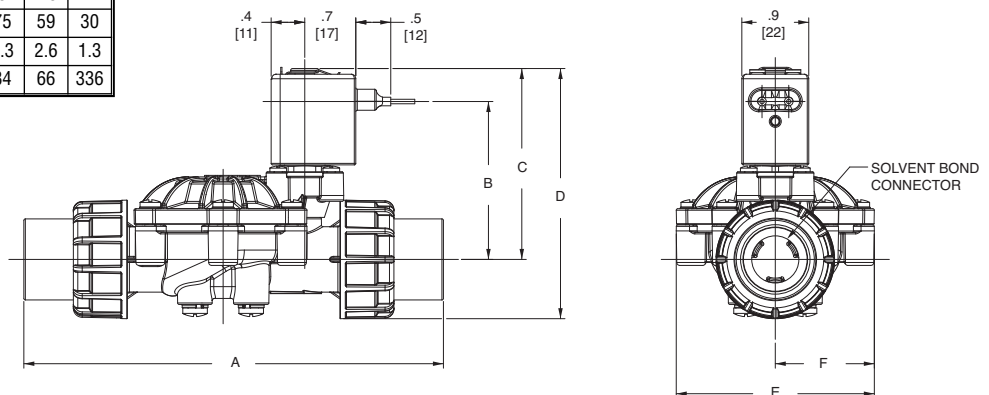
3/8" & 1/2" SOLVENT BOND CONNECTION WITH LEAD WIRE CONNECTION
