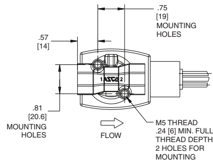
Const. Ref. 5, 6 (3/8" Pipe)
