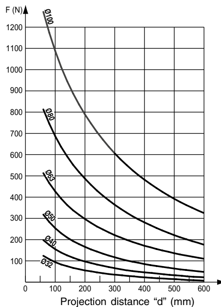
"H" GUIDING UNIT With slide bearings
