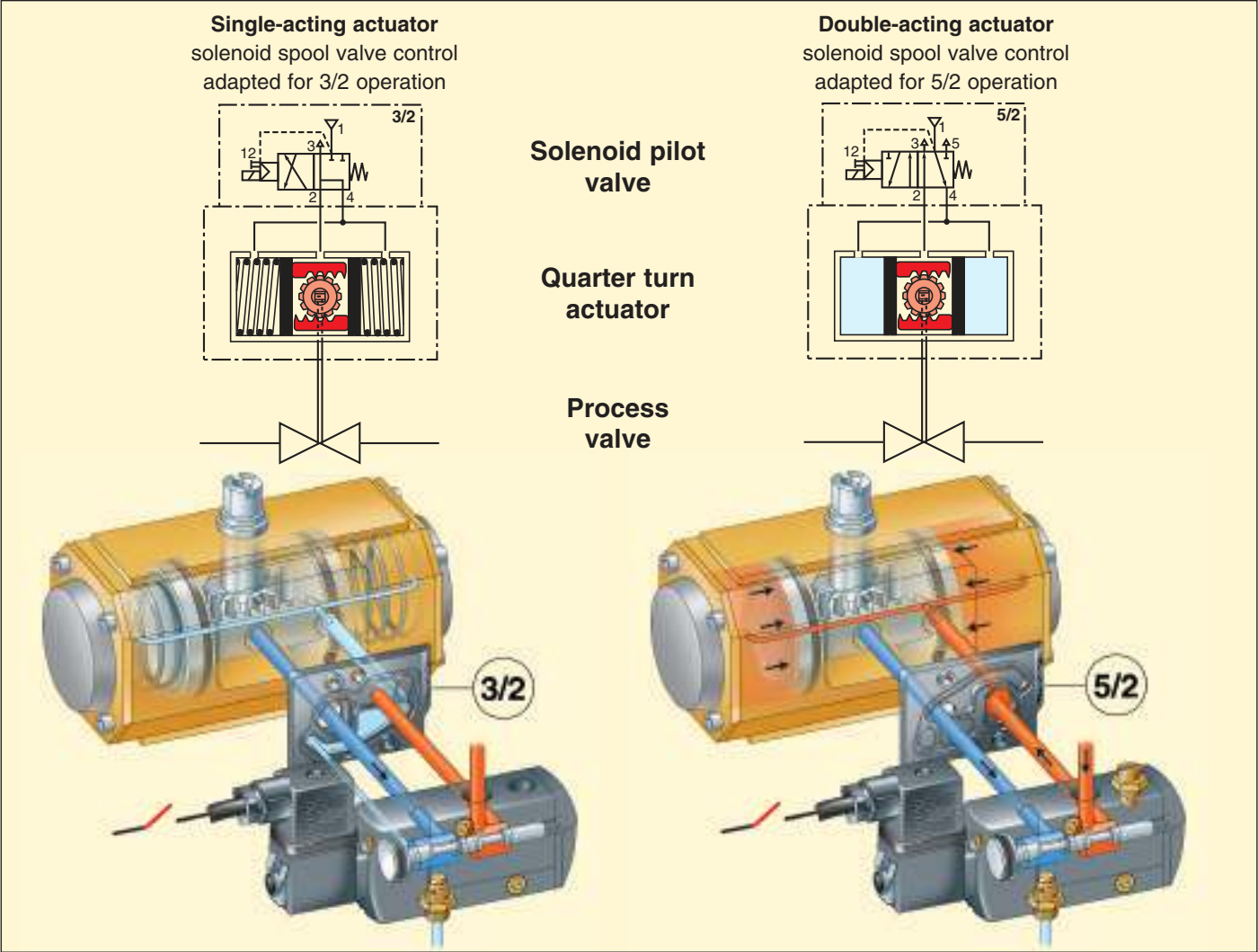
Single and Double acting actuators
