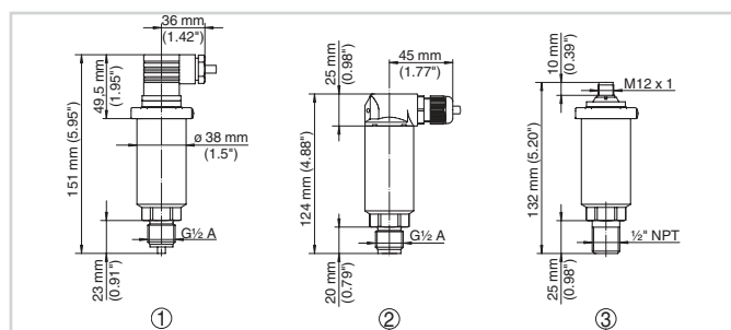
Dimensions VEGABAR 14
