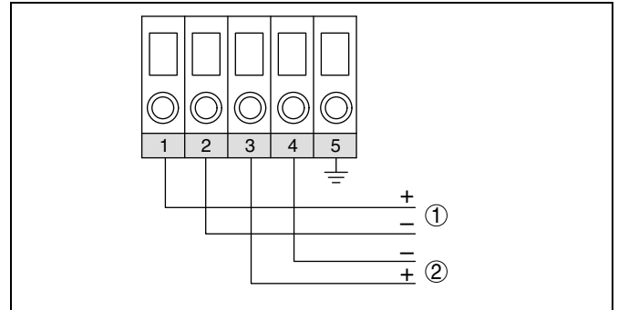
Fig. 18: Wiring plan, terminal housing
