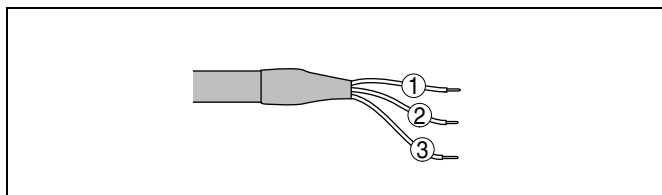
Fig. 16: Wiring plan cable outlet 3)
