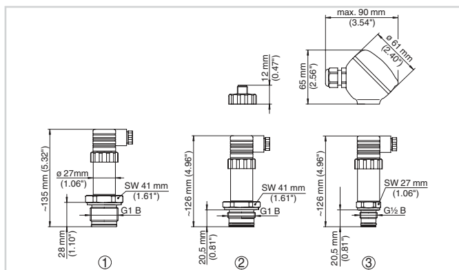
Dimensions VEGABAR 17
