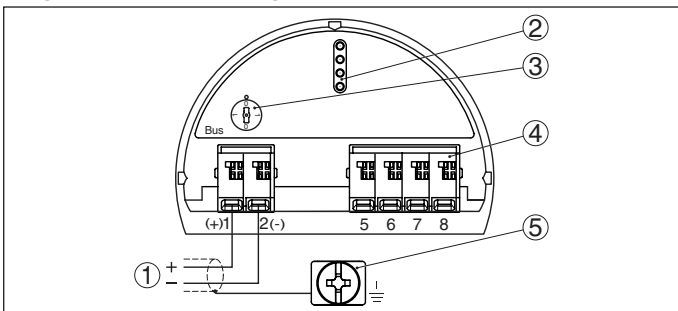
Fig. 30: Electronics and terminal compartment, single chamber housing
