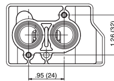
8551 NAMUR Footprint
