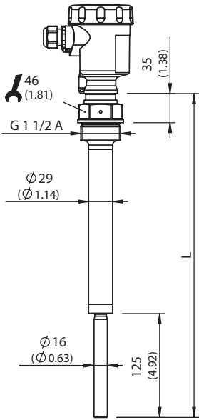
LBV331 threaded version G 1 1/2 A
