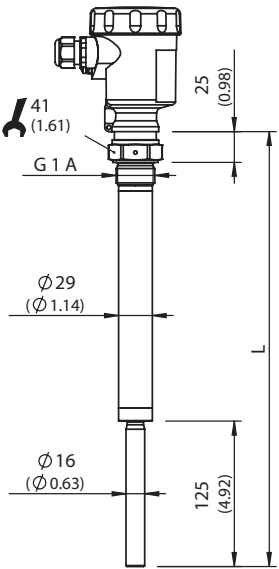
LBV331 threaded version G 1 A
