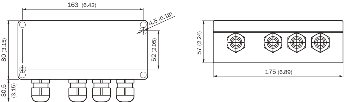
GM901 connection unit
