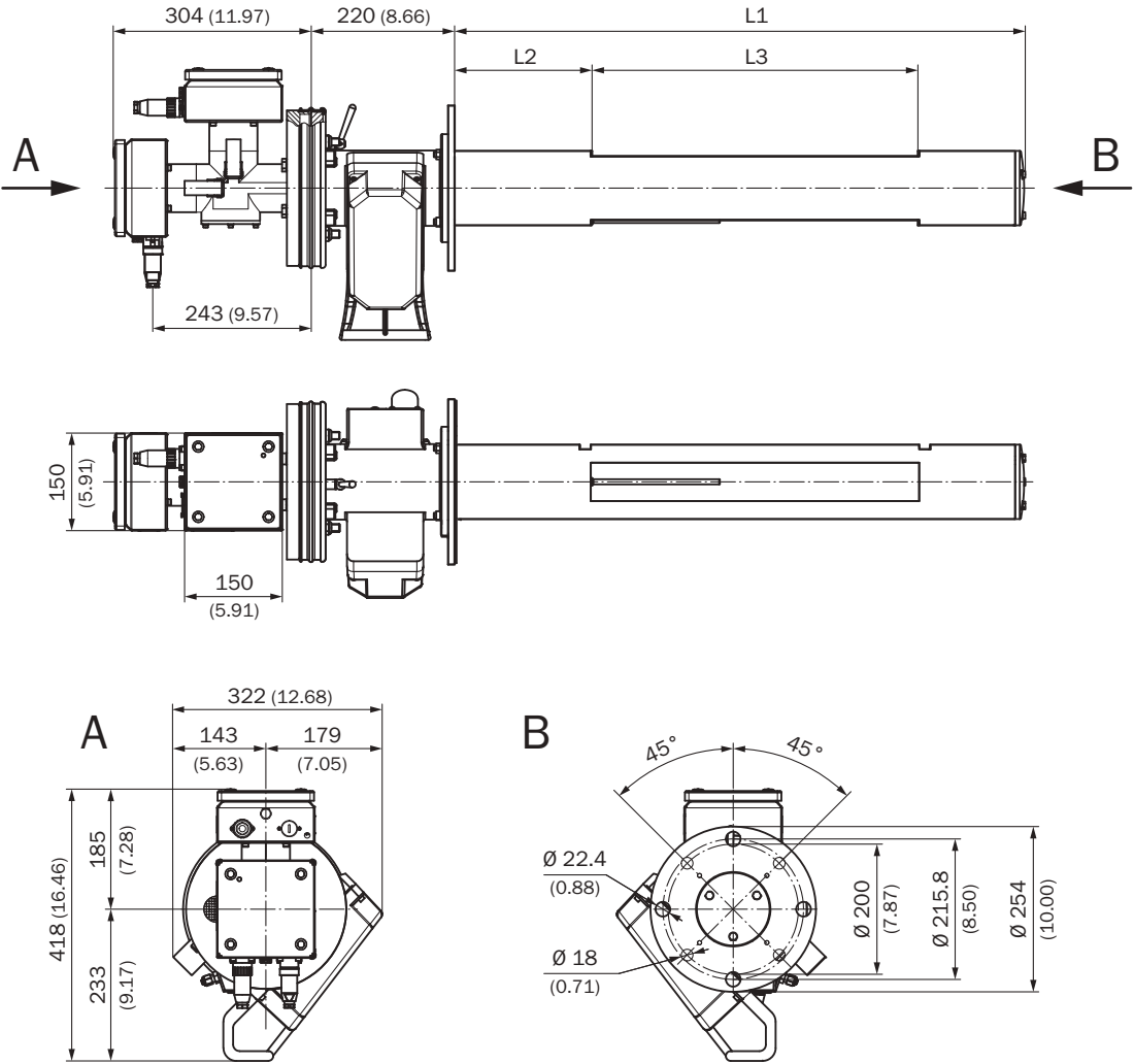
GM901 sender/receiver unit with open measuring probe (GMP)
