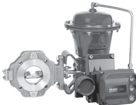
LUGGED STYLE (NPS 3 through NPS 12)
