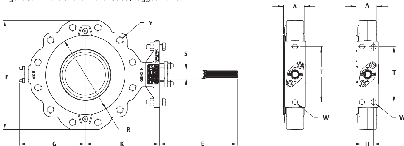
Figure 8. Dimensions for Fisher 8580, Lugged Valve
