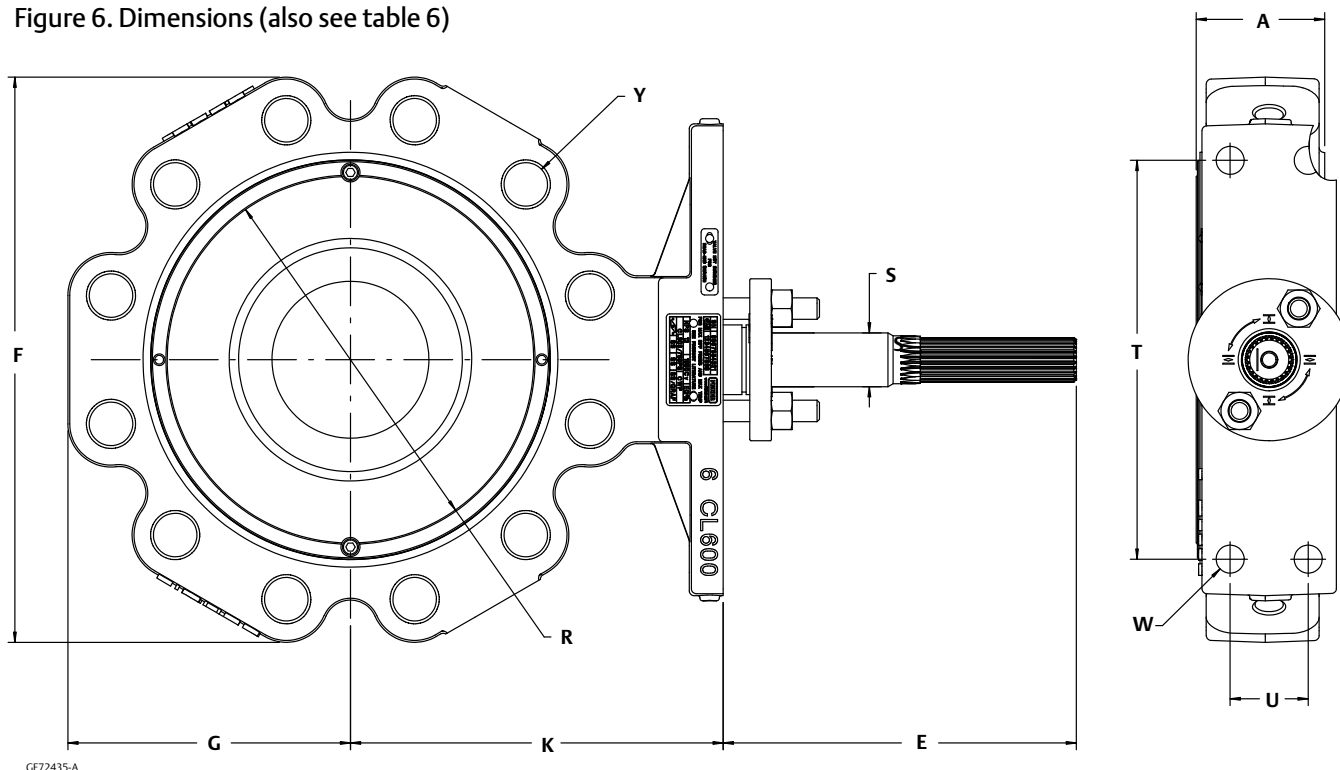
Figure 6. Dimensions (also see table 6)
