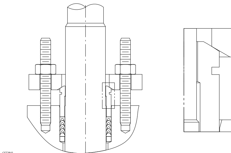
NPS 10 THROUGH 24 WITH STEPPED SHAFT
