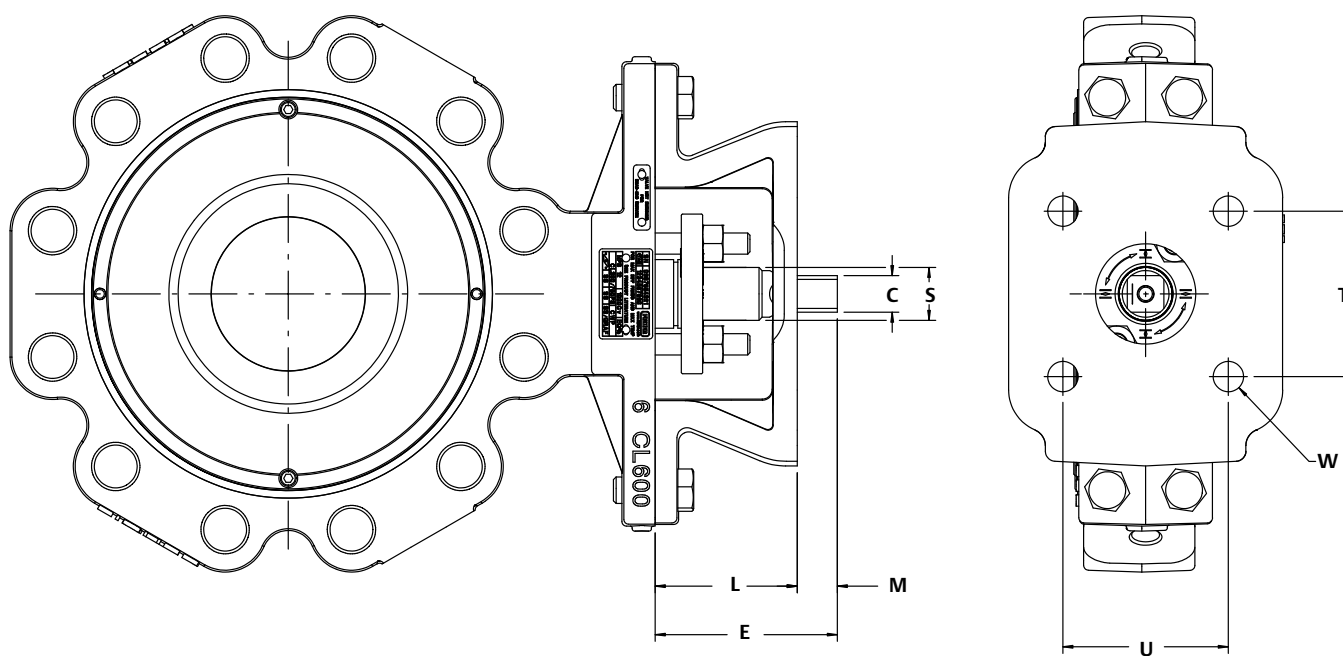
Figure 7. 8590 Valve Assembly with Mounting Bracket (also see table 7)
