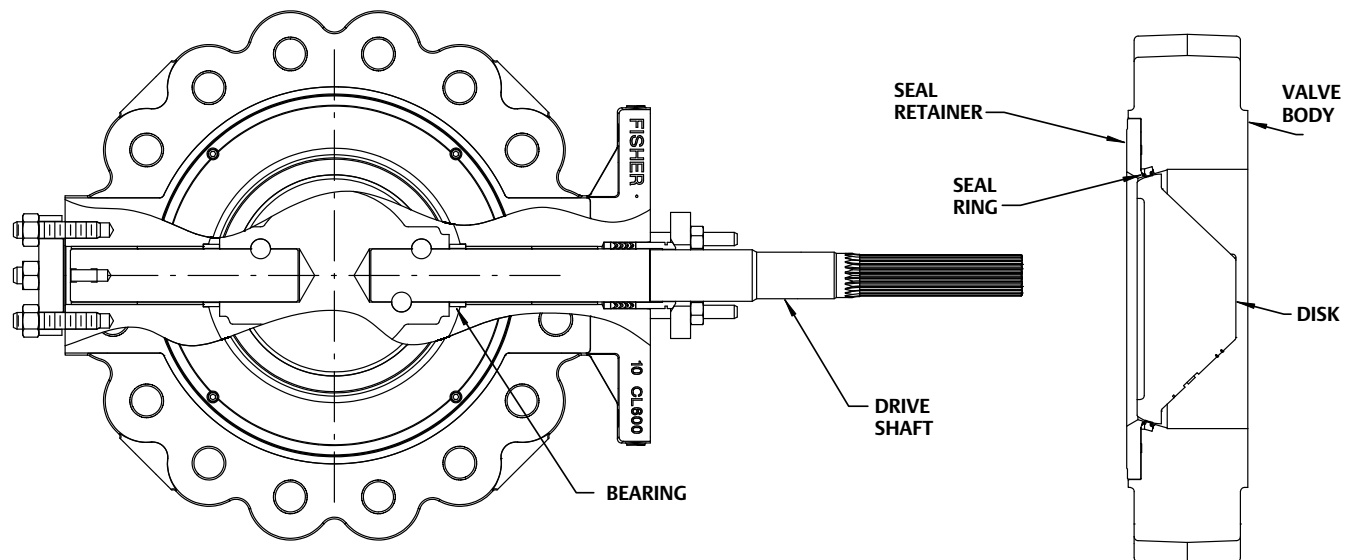
Figure 3. 8590, NPS 8 to 24, Valve Body Assembly
