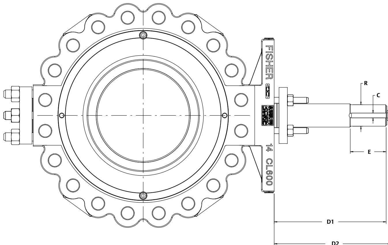
Figure 8. Dimensions for Fisher 8590 NPS 14 to 24 Valve with Keyed Shafts (also see table 8)
