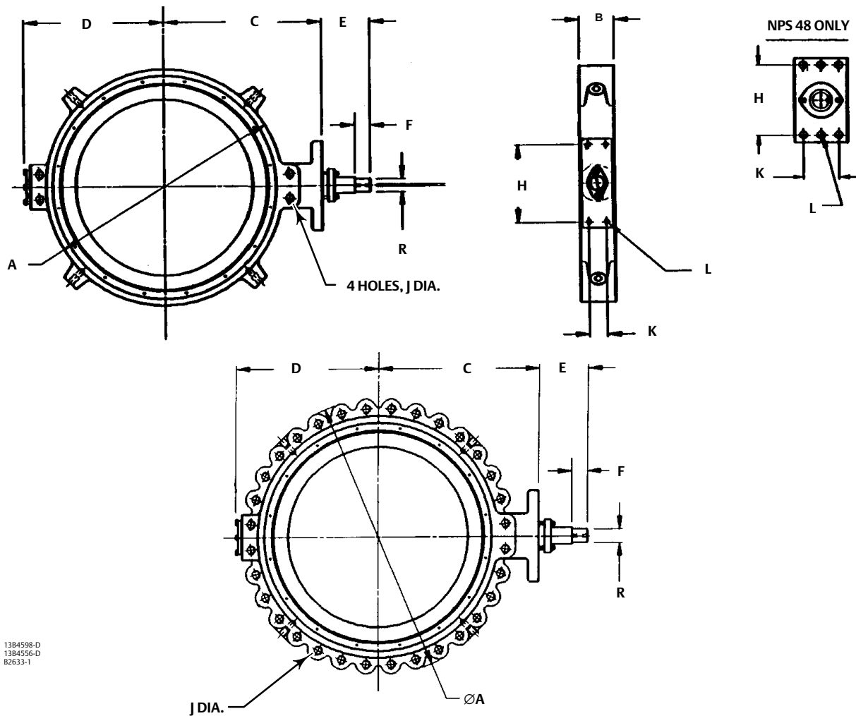
Figure 3. Dimensions Wafer and Single Flange Style CL150/150 (also see table 8)
