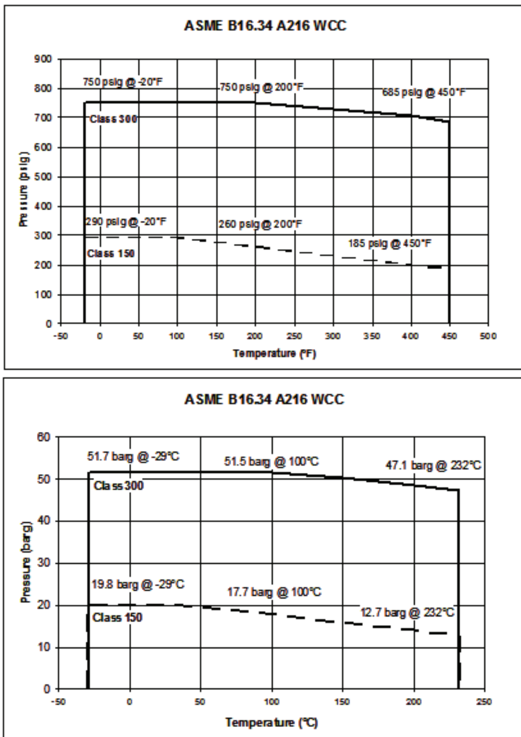
Figure 10. Baumann 24000CVF Carbon Steel Flanges, Pressure-Temperature Ratings
