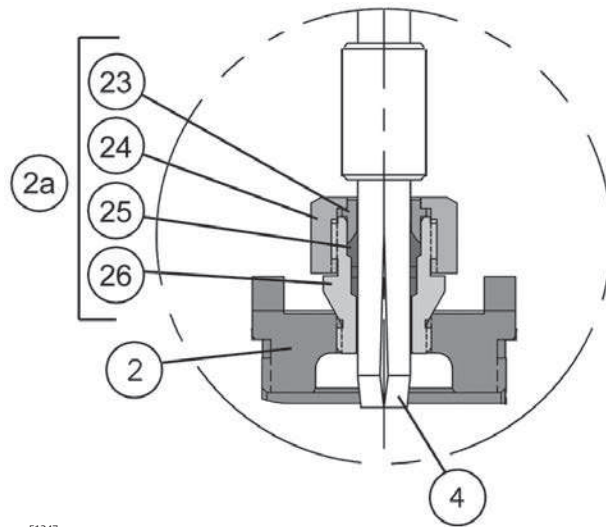
Figure 3. Optional 177 Low Flow Trim Assembly
