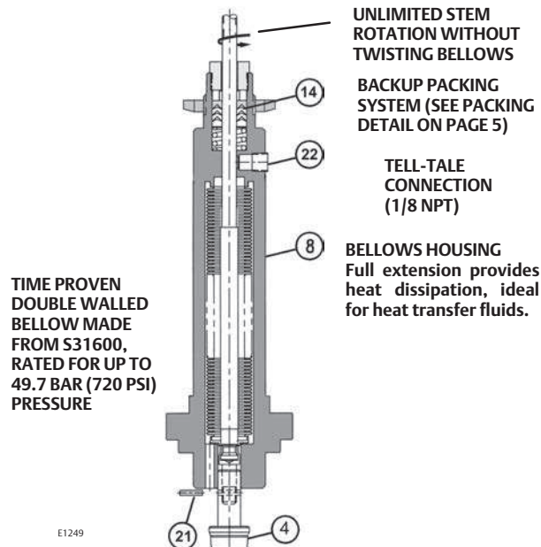
Figure 7. Baumann NOLEEK Bellow Bonnet Assembly
