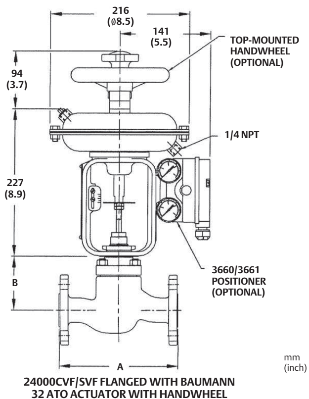
Figure 14. Dimensional Drawings
