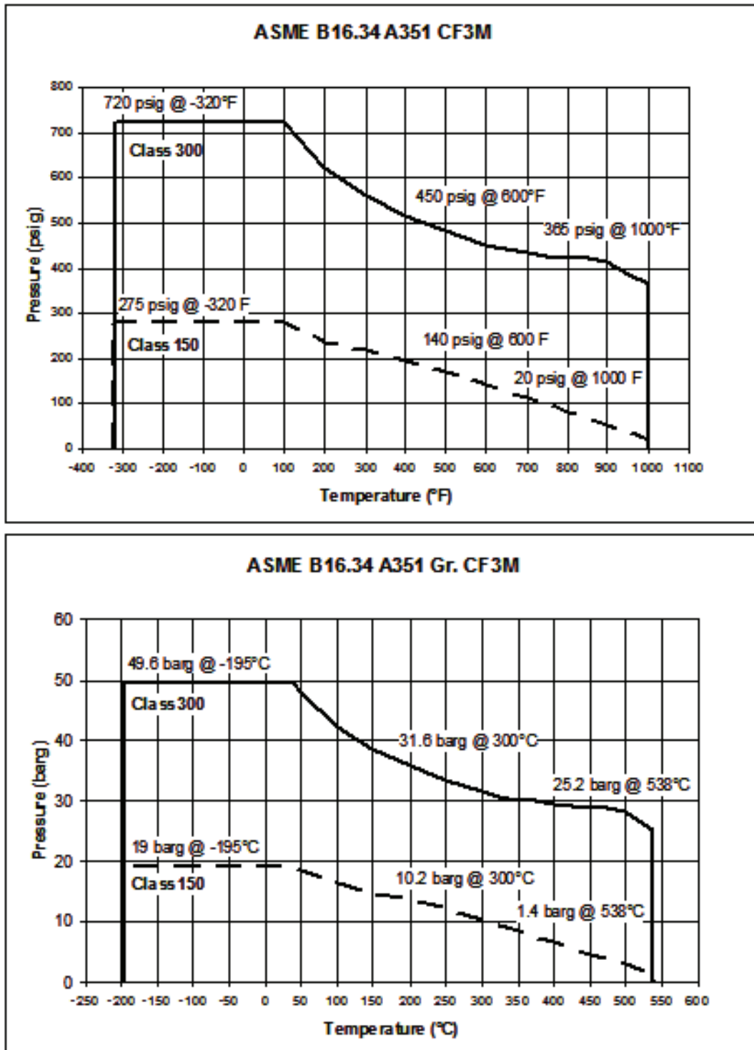
Figure 11. Baumann 24000SVF Stainless Steel Flanges, Pressure-Temperature Ratings
