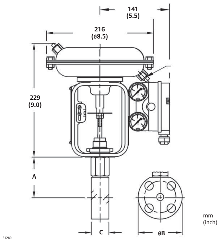
BAUMANN 32 ACTUATOR WITH FISHER 3660/3661 POSITIONER
