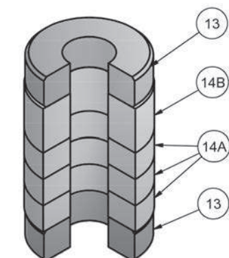
Figure 6. Molded Graphite (Flexible Graphite) Packing Kit (Optional)
