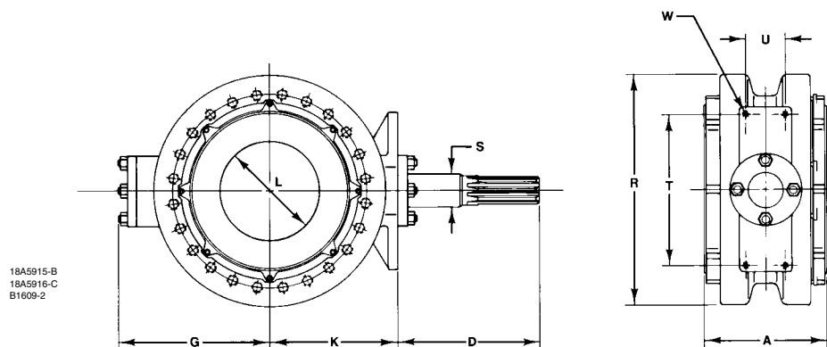
NPS 20 AND 24
