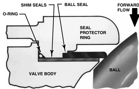
BALL SEAL
