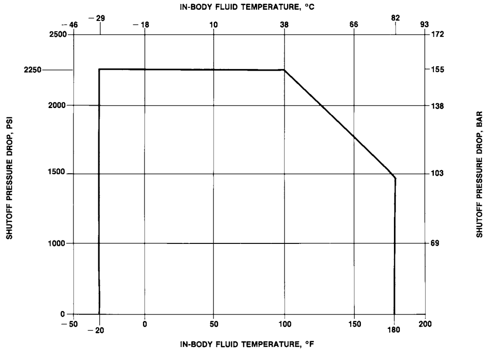
Figure 3. Maximum Allowable Shutoff Pressure Drop for Single and Dual POM Seal Construction
