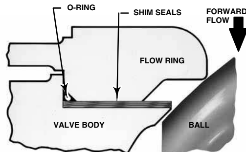
FLOW RING
