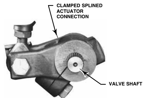
Figure 6. Clamped Splined Actuator Connection on Type 1061 Actuator
