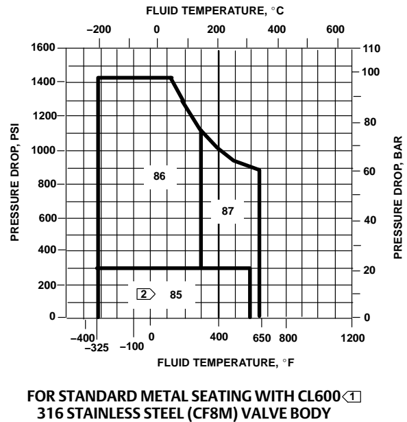
Figure 11. Typical Trim Used for NACE MR0175 / ISO 15156 and NACE MR0103. Environmental restrictions may apply
