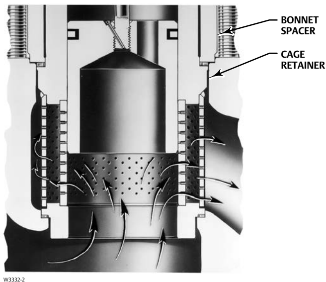
Figure 8. Whisper Trim III Cage in Fisher ED Valve
