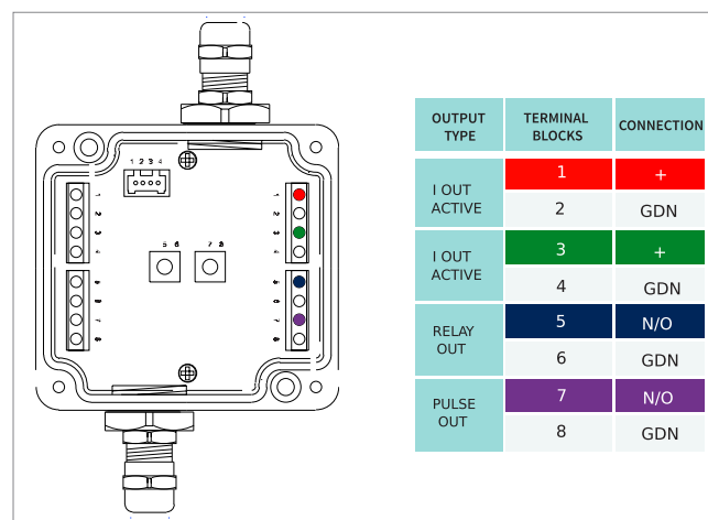
7. Input/output box, connection terminals
