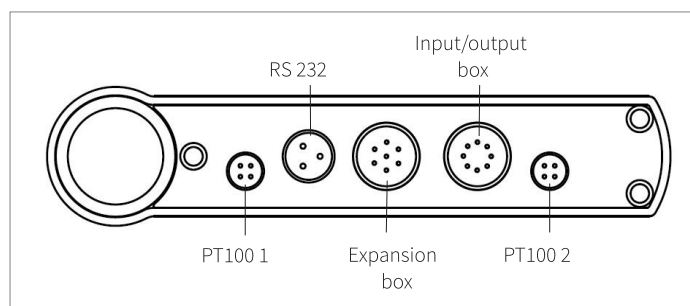
6. Bottom connectors
