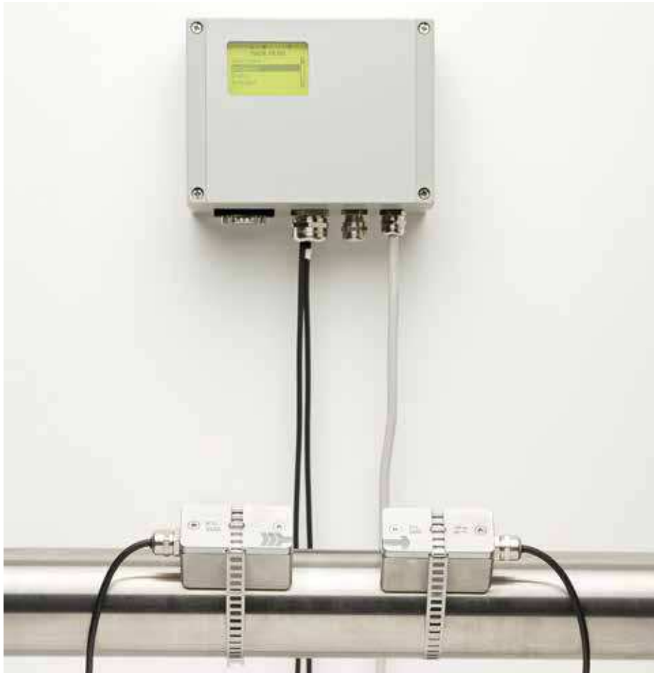
The KATflow 100 and K1L transducers for installation on standard process applications with pipes greater than 50 mm.
